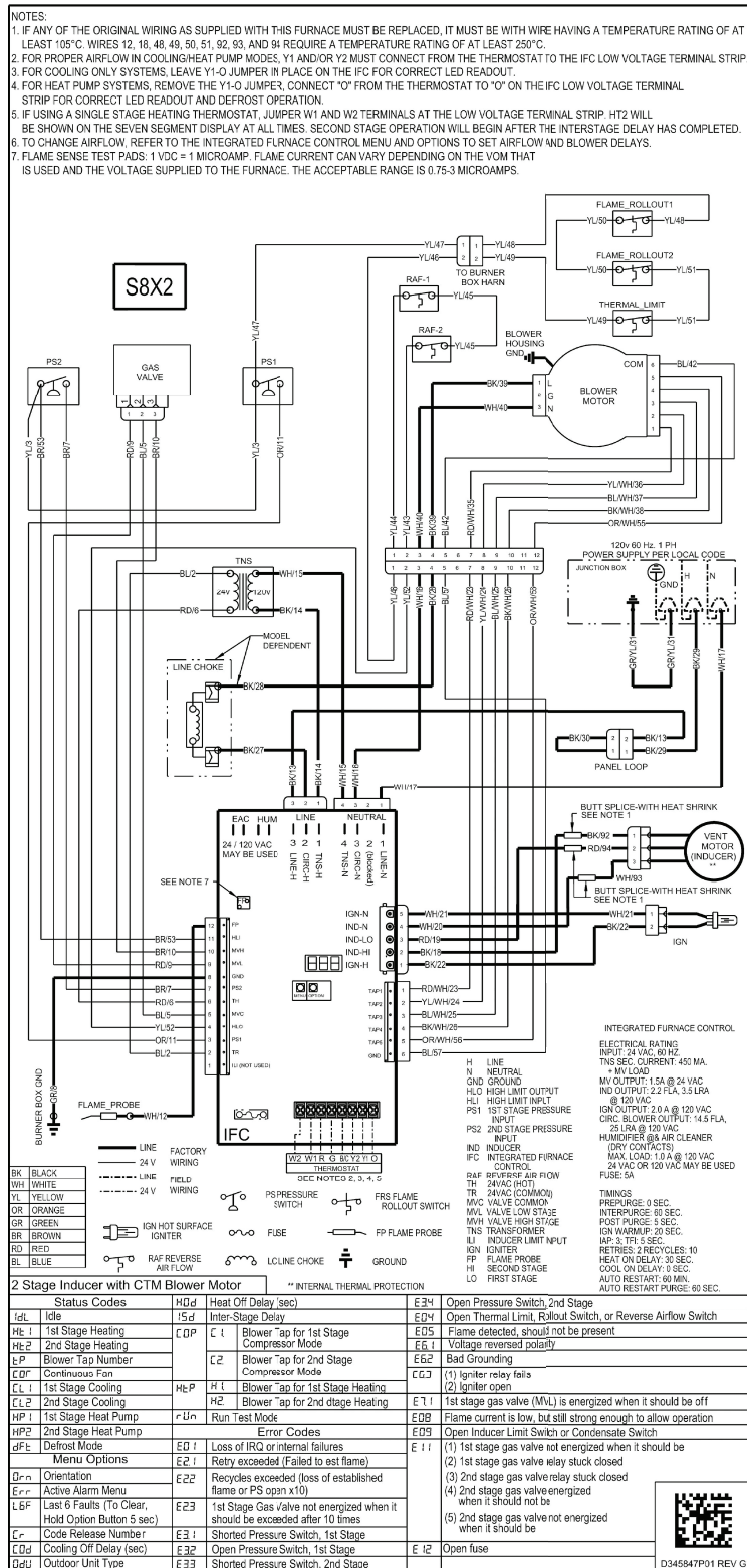
Figure 5. S8X2 — wiring diagram
