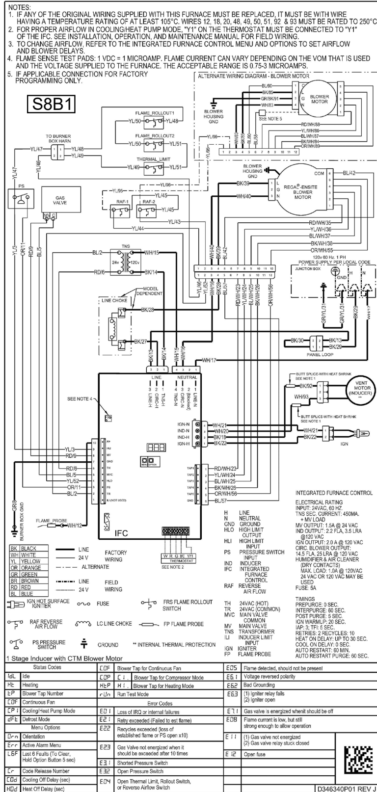
Figure 1. S8B1 – wiring diagram
