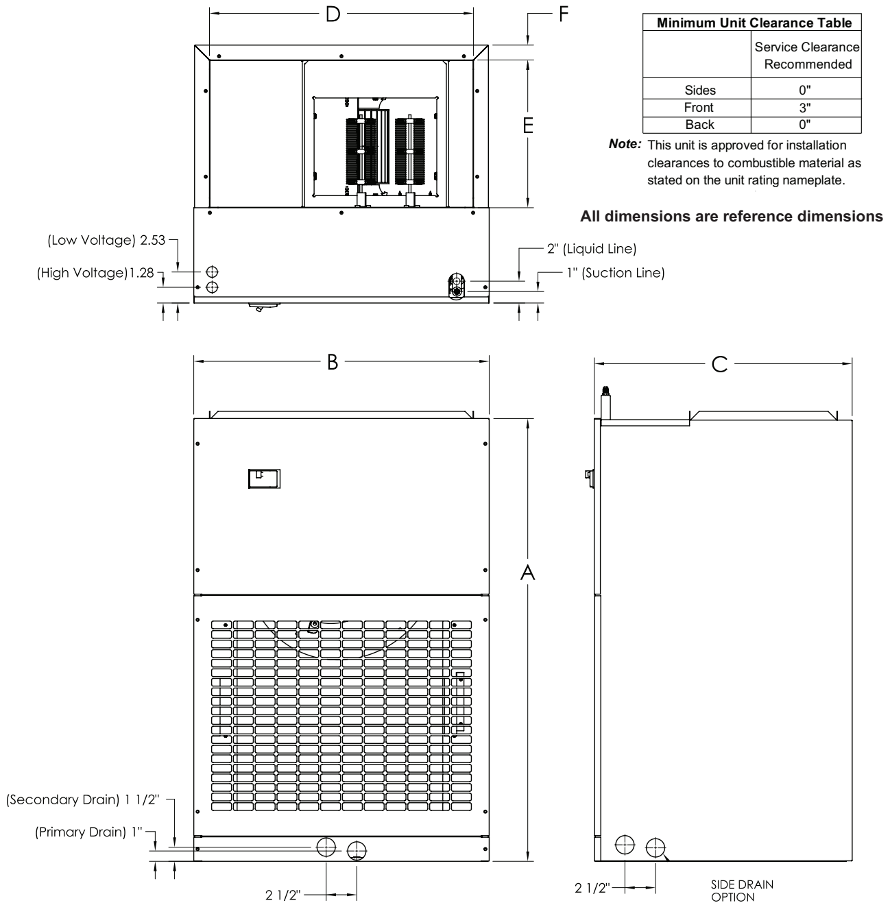
Figure 2. 5TMM5BOA30M21SA and 5TMM5BOC36M31SA
