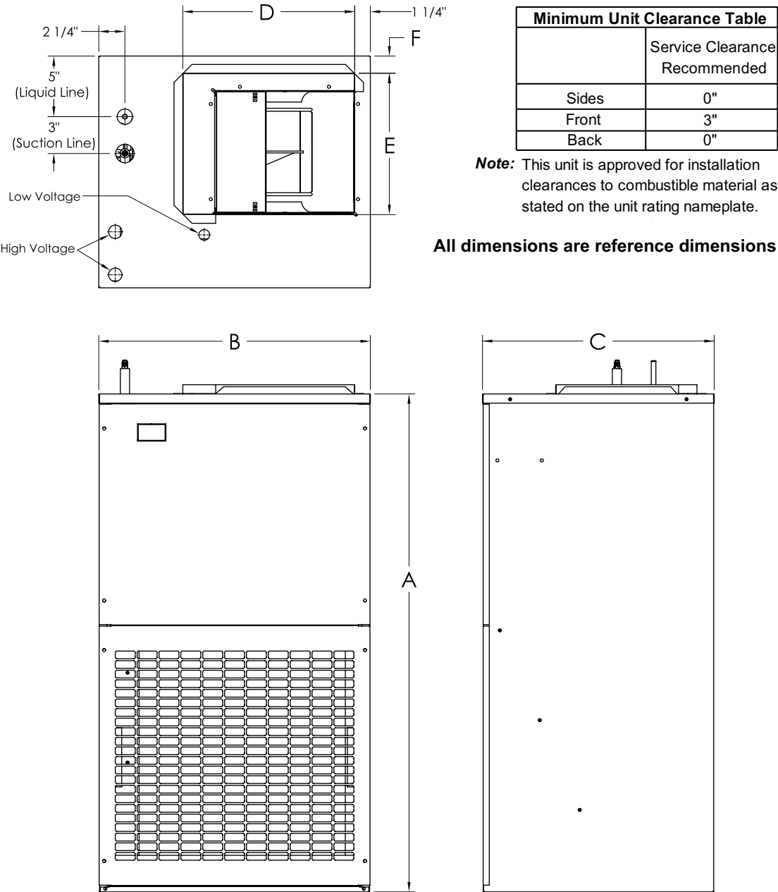
Figure 1. 5TMM5BOB30M21SA and 5TMM5BOB36M31SA
